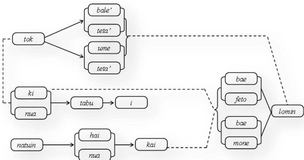
Figure 5. Cognitive Map 2
